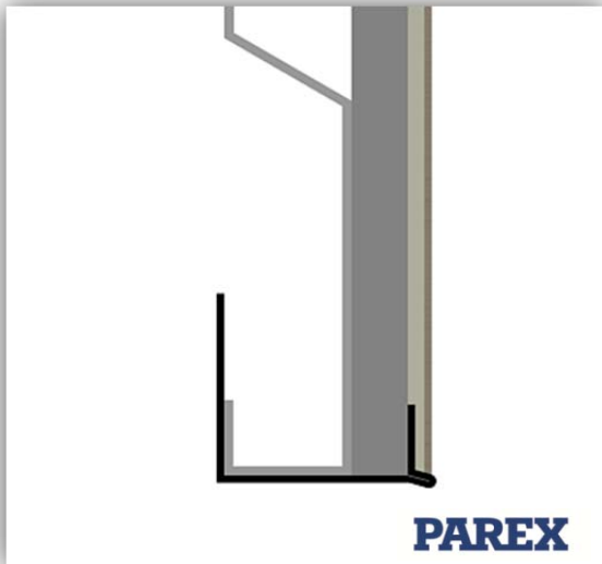
Parexdirect Acrylic System 6mm Base Rail
