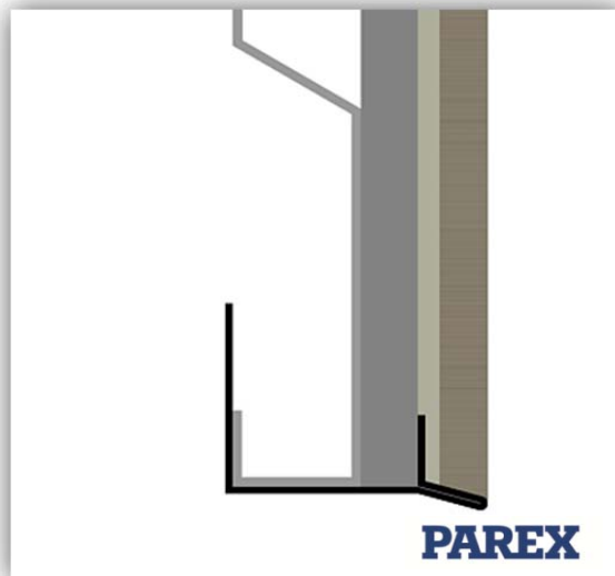
PAREXDIRECT Mineral System 15mm Base Rail
