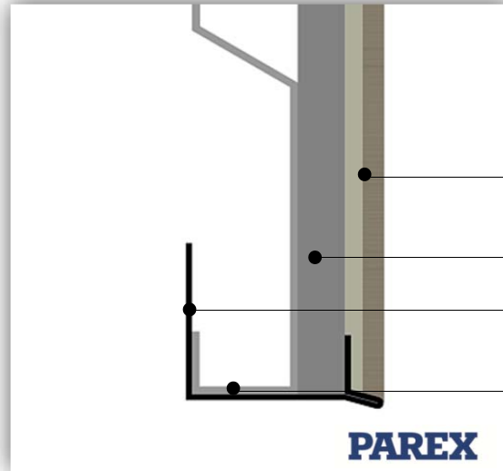
Parexdirect Marbri System 10mm Base Rail
